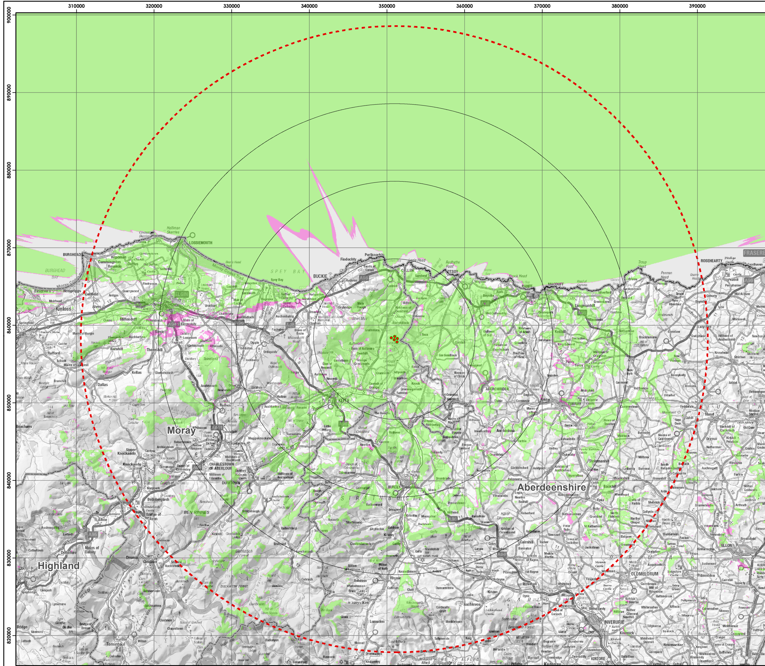
Figure 3 Comparative Blade Tip ZTV
